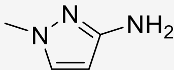
3-Amino-1-methylpyrazole
