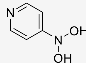
N-hydroxy-N-(pyridin-4-yl)hydroxylamine
