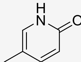
5-Methyl-2-pyridone
