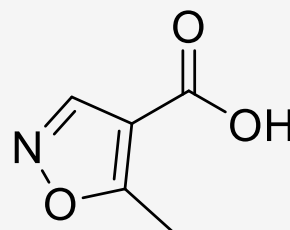
5-Methyl-1,2-oxazole-4-carboxylic acid
