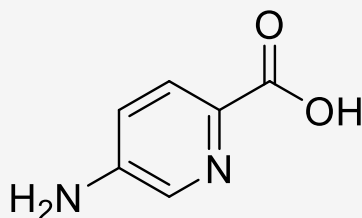
5-Aminopicolinic acid
