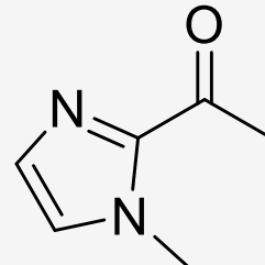
1-(1-methyl-1H-imidazol-2-yl)ethan-1-one
