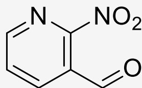
2-nitronicotinaldehyde
