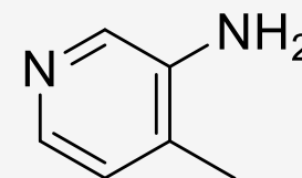
4-methylpyridin-3-amin
