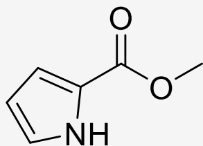
Methyl 2-pyrrolecarboxylate
