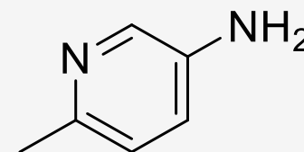
6-Methylpyridin-3-amine
