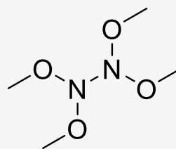
Tetramethoxyhydrazine
