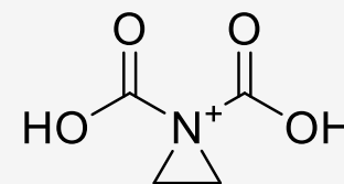
aziridin-1-ium-1,1-dicarboxylic acid
