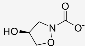
(4S)-4-hydroxy-1,2-oxazolidine-2-carboxylate
