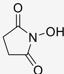
1-hydroxypyrrolidine-2,5-dione
