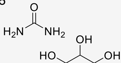
Urea / Glycerol
