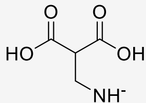
2,2-dicarboxyethylazanide
