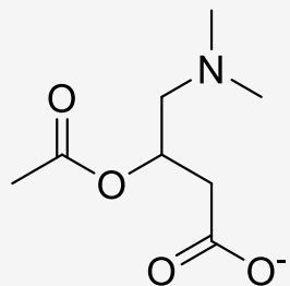
Acetyl-L-Carnitine Hydrochloride
