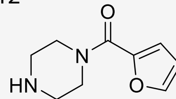
furan-2-yl(piperazin-1-yl)methanone
