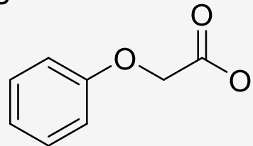
2-phenoxyacetate
