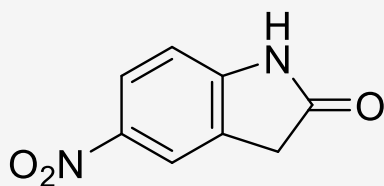
5-nitroindolin-2-one
