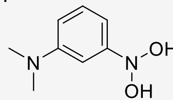
3-(dihydroxyamino)-N,N-dimethylaniline
