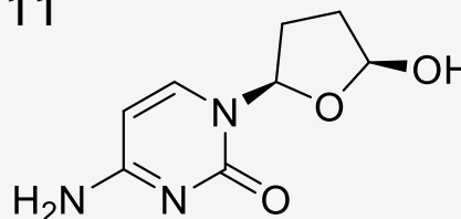
4-amino-1-((2R,5S)-5-hydroxy tetrahydrofuran-2-yl)pyrimidin-2(1H)-one
