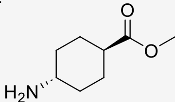
Methyl trans-4-Aminocyclohexanecarboxylate
