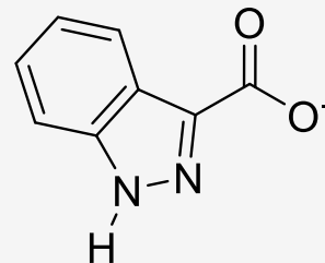
1H-indazole-3-carboxylate
