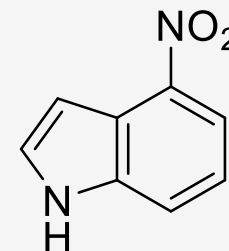
4-nitro-1H-indole
